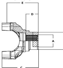
Pinion Yoke
