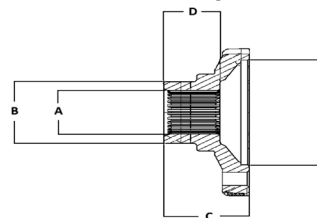
Pinion Flange
